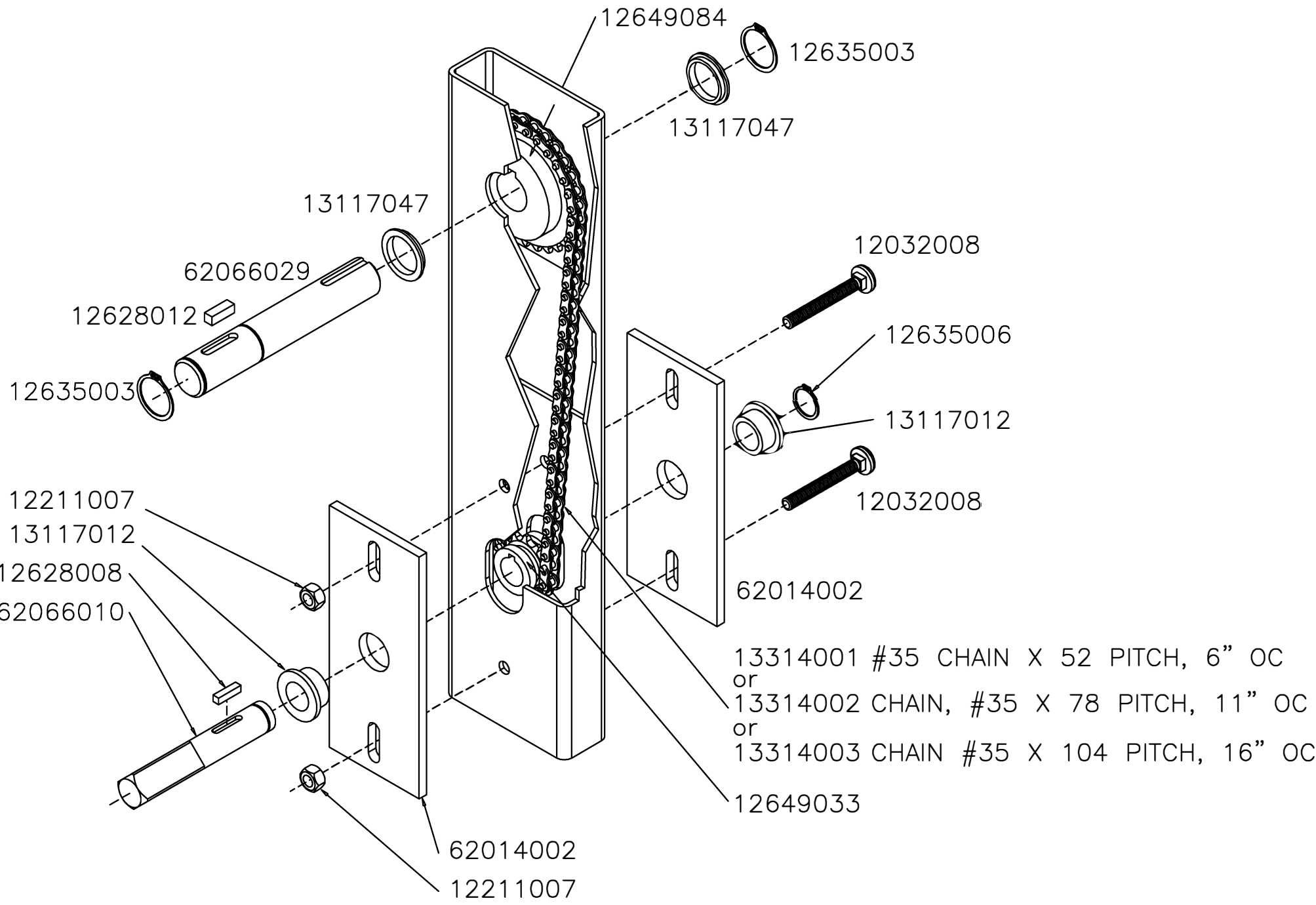
CONTROL PANEL REDUCER ASSEMBLY, MILLENNIUM EDITION
